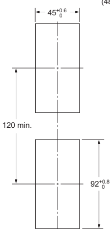
Mounted Separately
