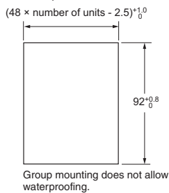
Group Mounted
